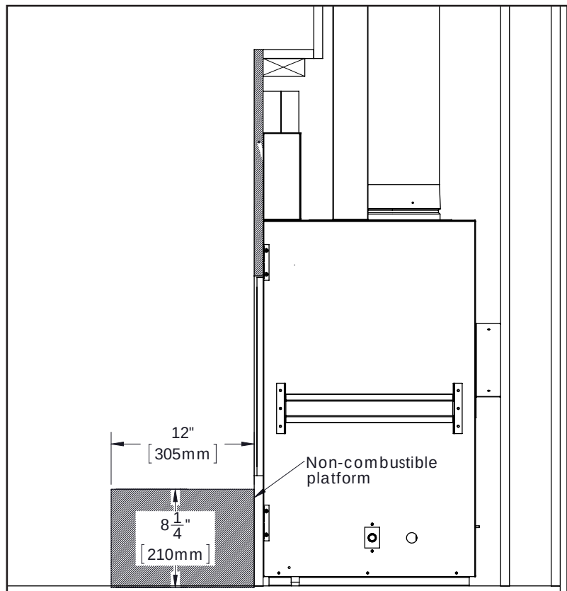
Figure 35: Non-Combustible Platform
