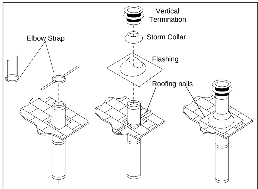
Figure 49. Vertical Vent Termination
