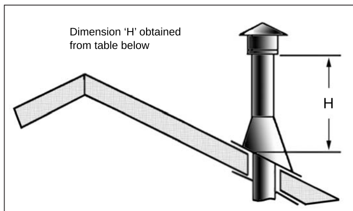
Figure 50: Height of Vertical Termination; Reference Table 8
