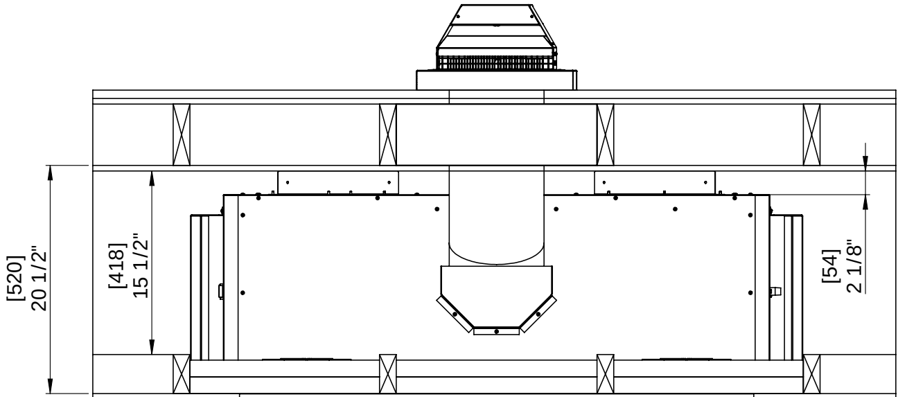
Figure 40(a). Dimensions for a Horizontal Installation
