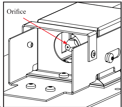
Figure 10: Orifice location
