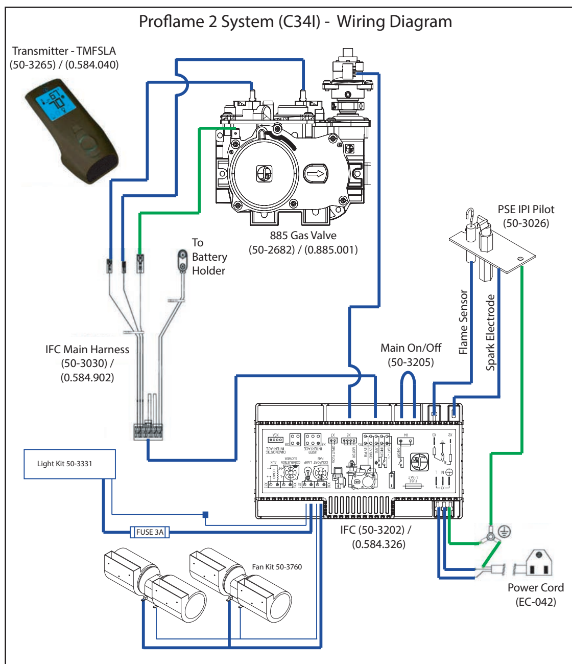
Figure 54: C34I Wiring Diagram
