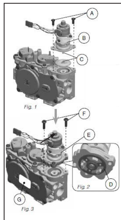
Figure 11: 885 Gas Valve
