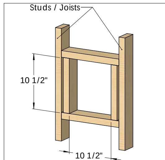
Figure 43. Vent Framing For Wall or Ceiling
