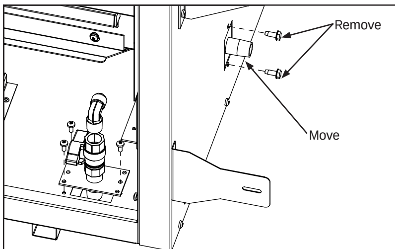
Figure 33: Alternate Gas Inlet Location
