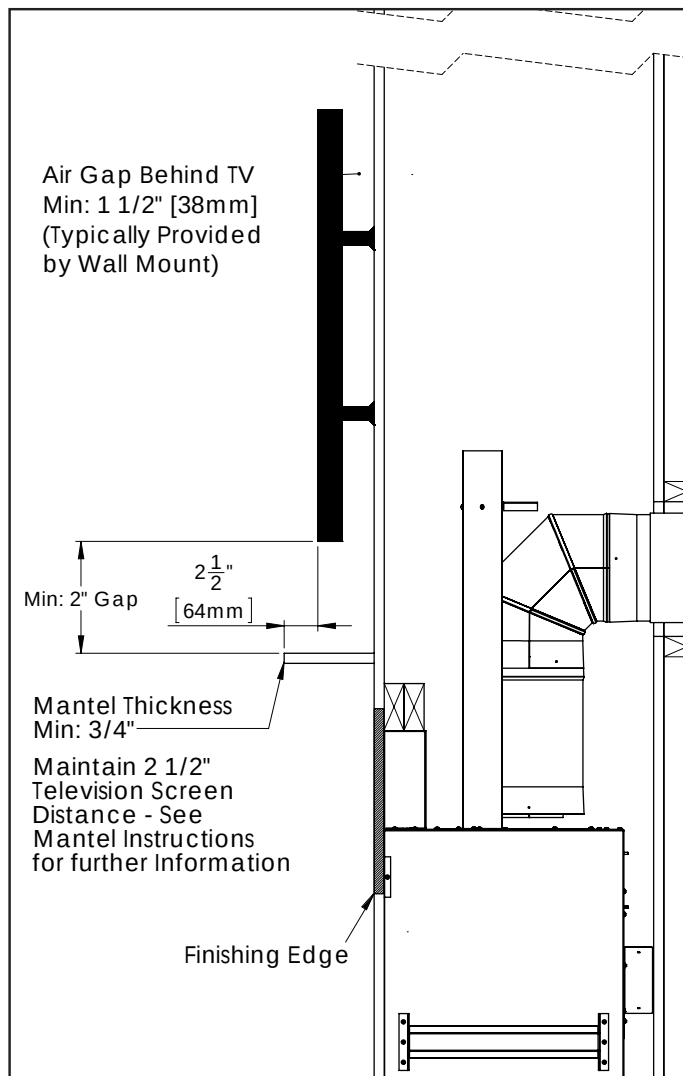
Figure 41(a). Minimum TV Install Clearances
