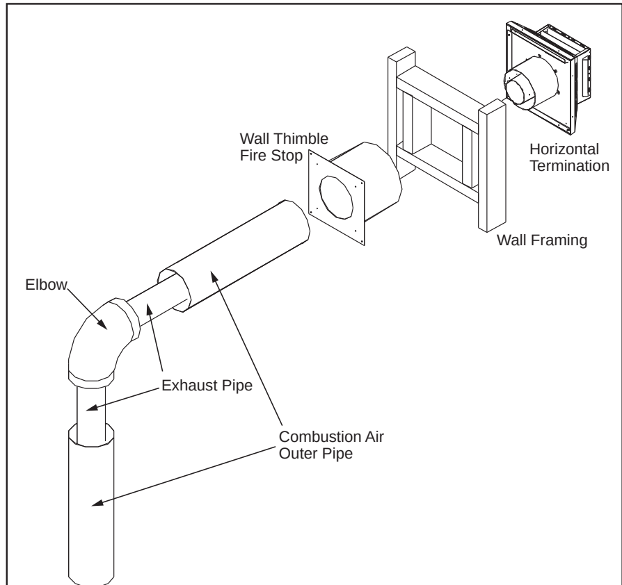
Figure 48. Horizontal Vent Termination
