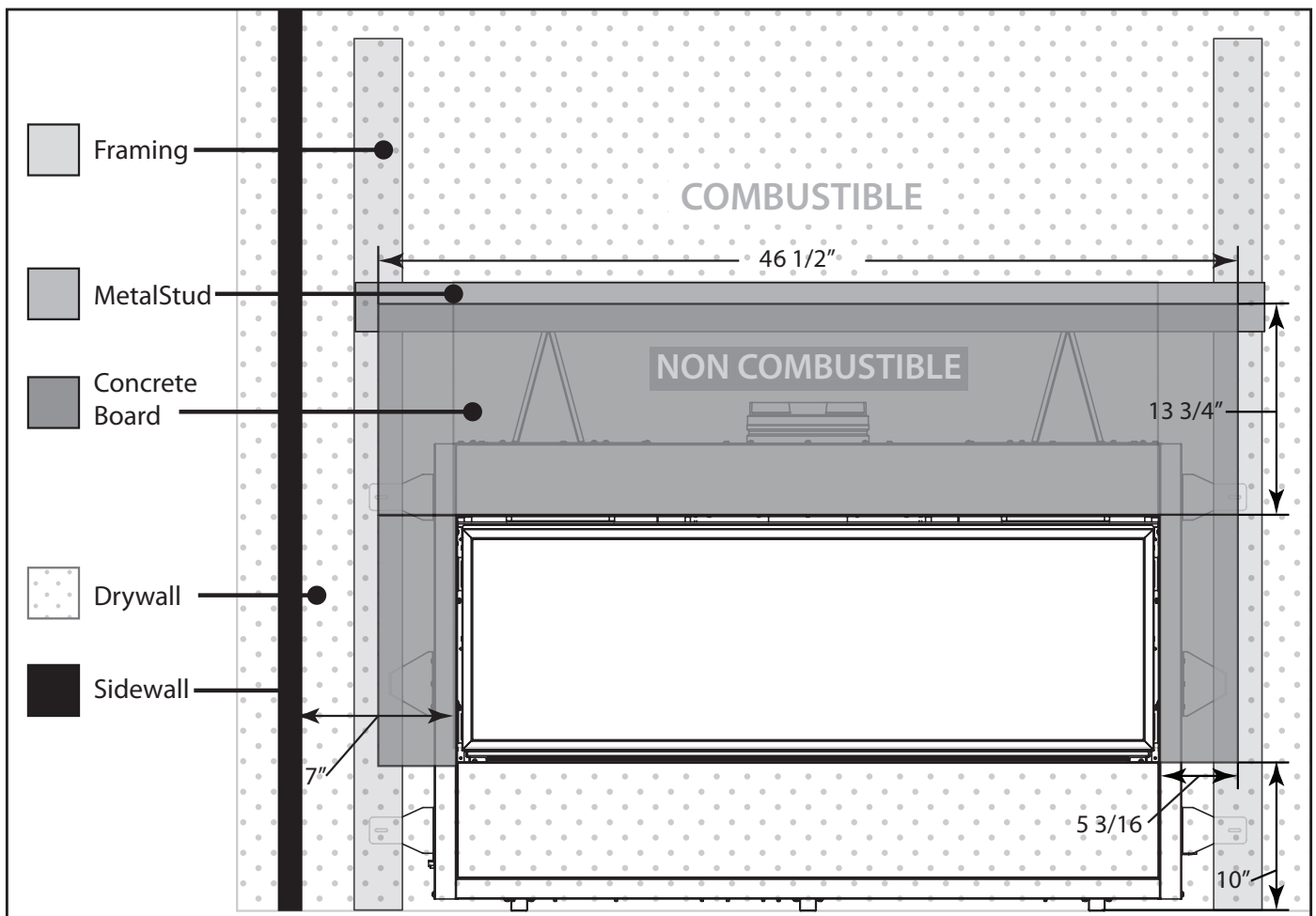
Figure 19. Finishing Non-Combustible Zone
