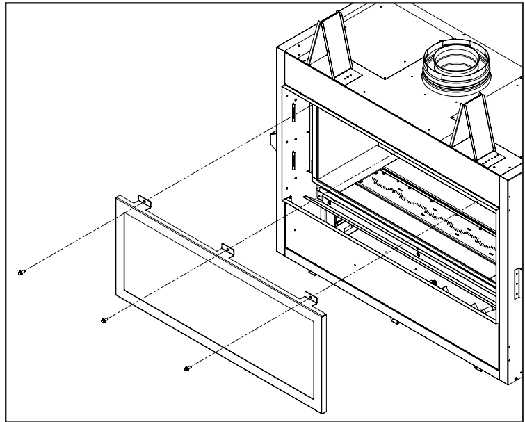
Figure 5. Door Removal Motion
