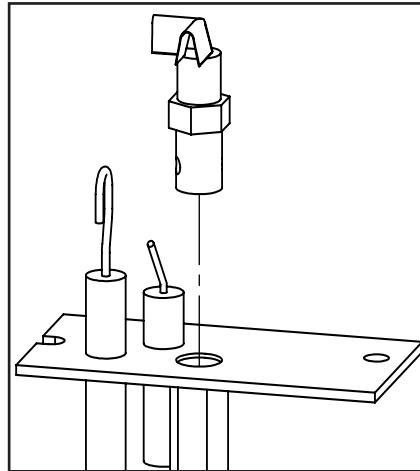
Figure 9. Pilot Orifice
