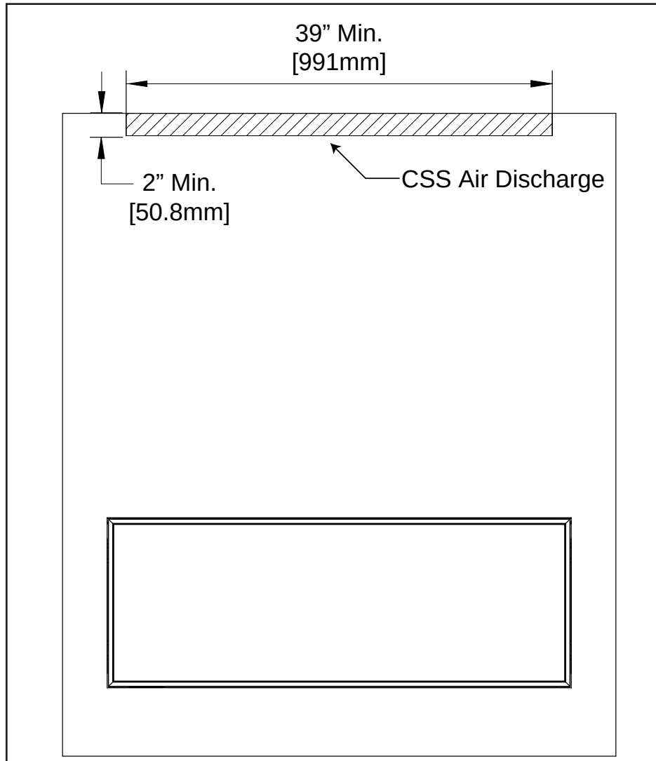
Figure 24 CSS Outlet
