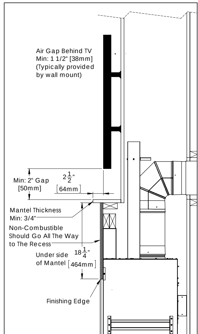
Figure 41(b). Recess Minimum TV Install Clearances
