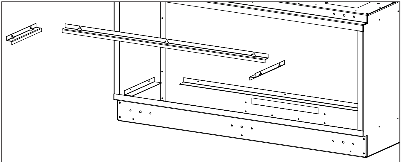
Figure 60: Panel Installation
