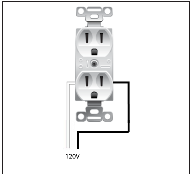
Figure 55: C34I Receptacle Wiring
